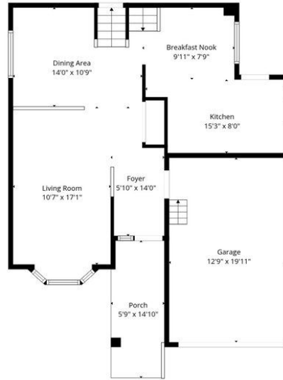
Floor 3
