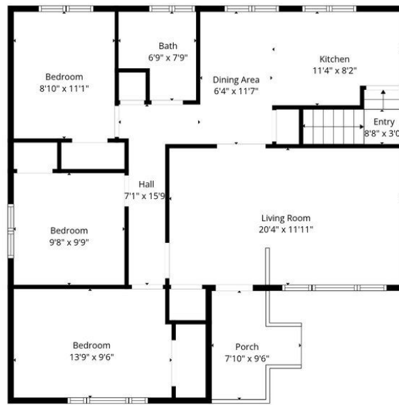
Floor 2
